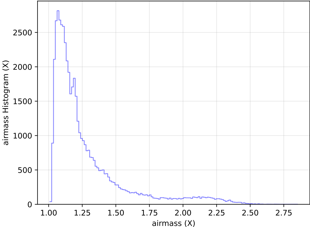
too_elab_r8_d2_griz_v3.4_10yrs Yr 1 r band: airmass Histogram
