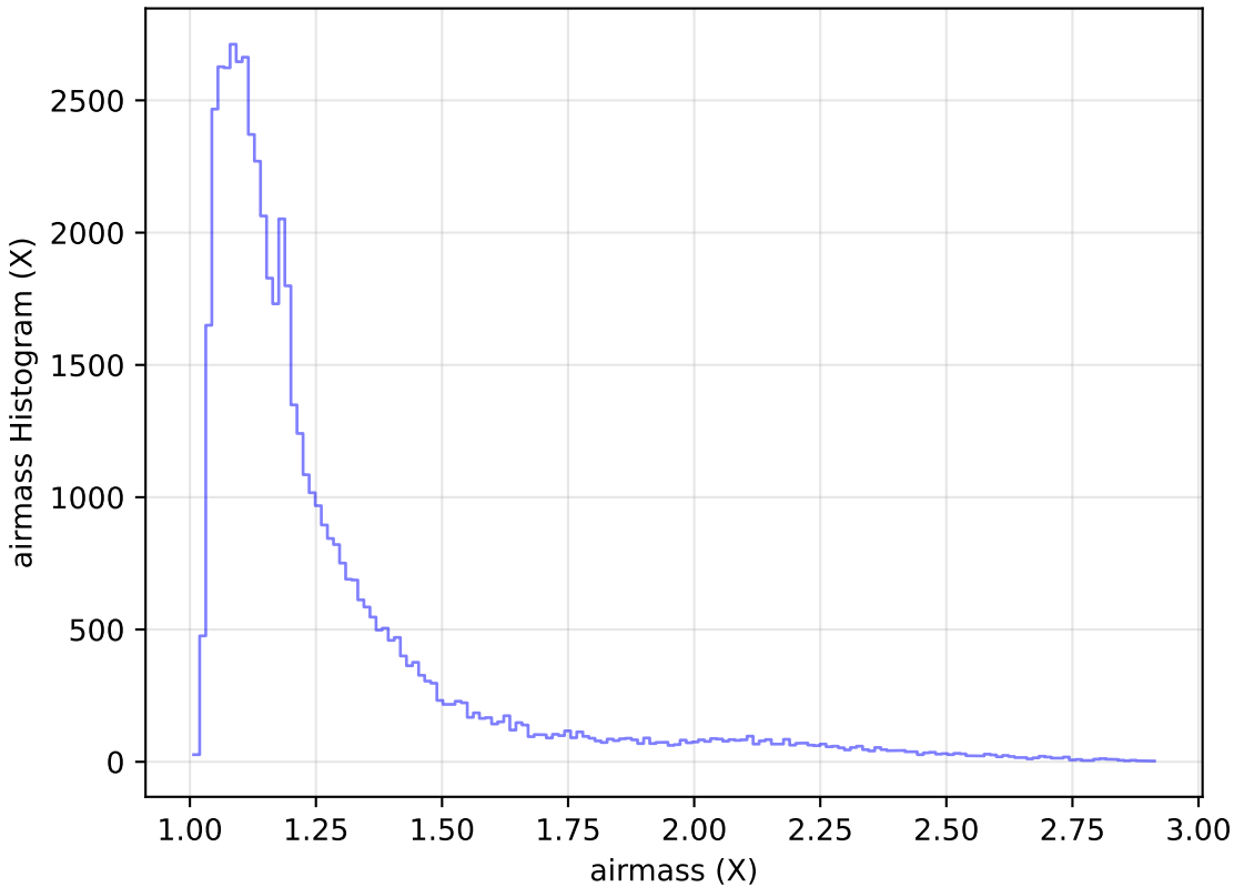
too_elab_r8_d2_griz_v3.4_10yrs Yr 1 i band: airmass Histogram
