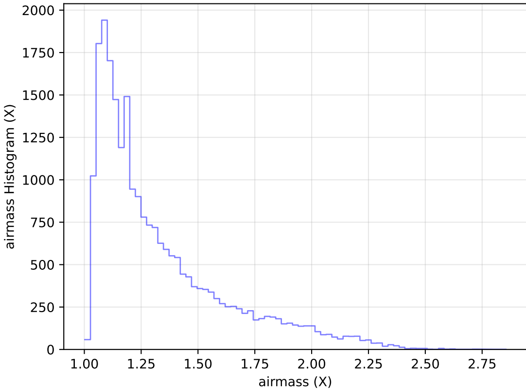
too_elab_r8_d2_griz_v3.4_10yrs Yr 1 g band: airmass Histogram
