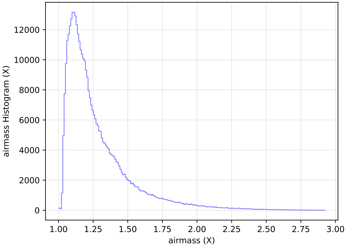
too_elab_r8_d2_griz_v3.4_10yrs WFD y band: airmass Histogram
