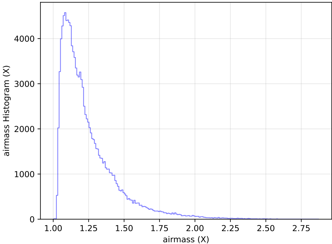
too_elab_r8_d2_griz_v3.4_10yrs WFD u band: airmass Histogram
