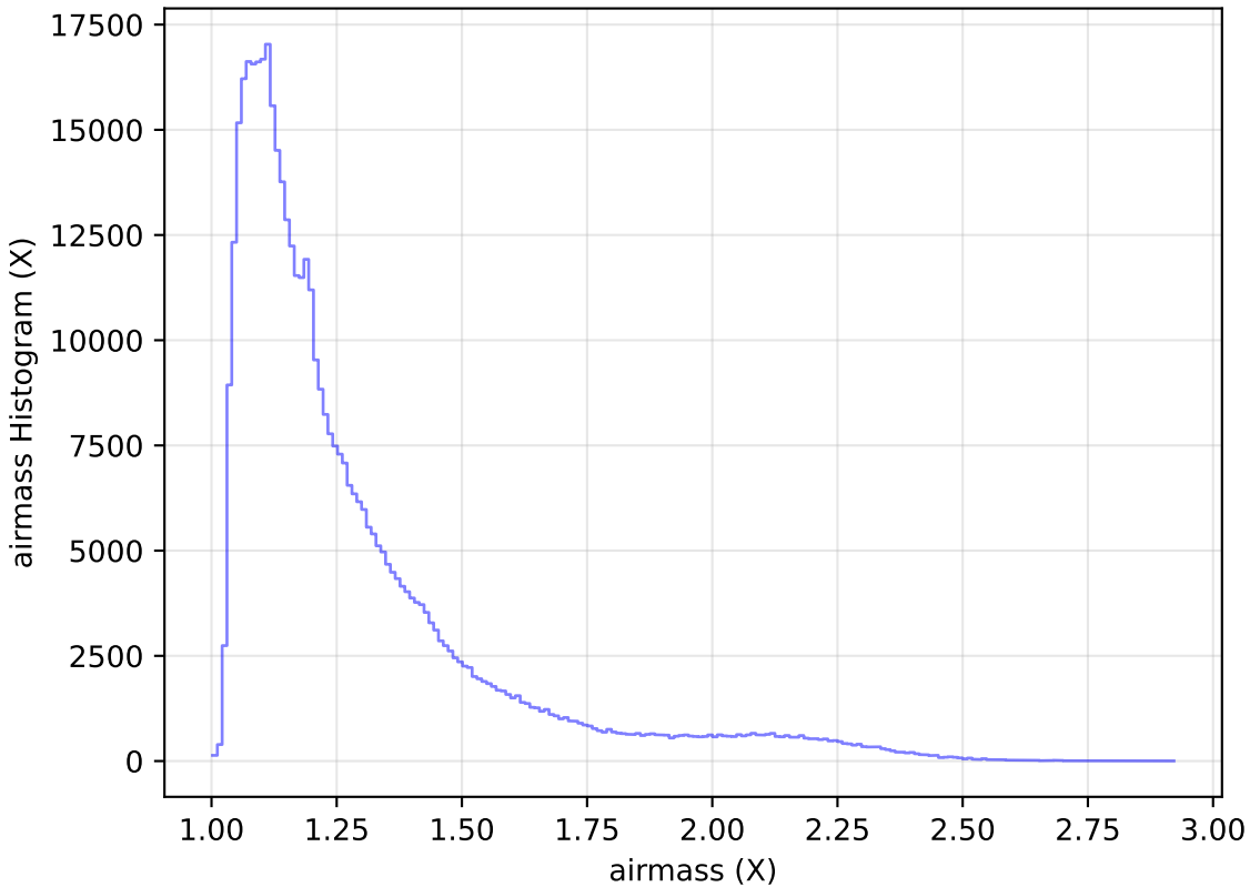
too_elab_r8_d2_griz_v3.4_10yrs WFD r band: airmass Histogram
