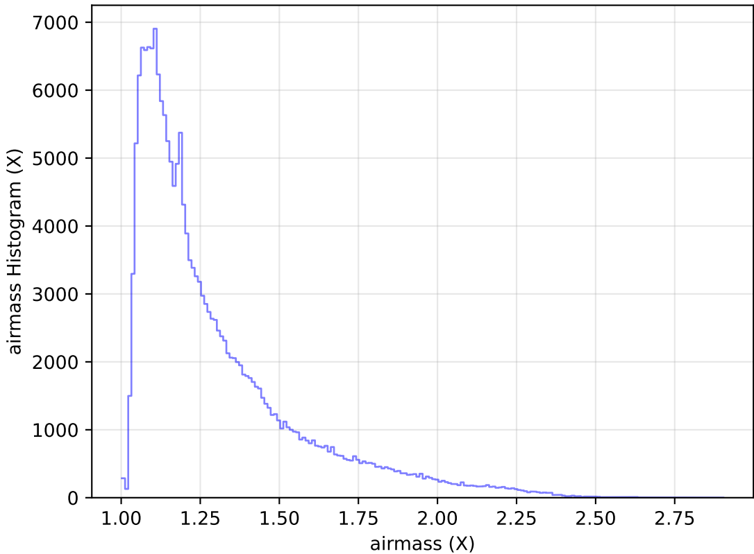
too_elab_r8_d2_griz_v3.4_10yrs WFD g band: airmass Histogram
