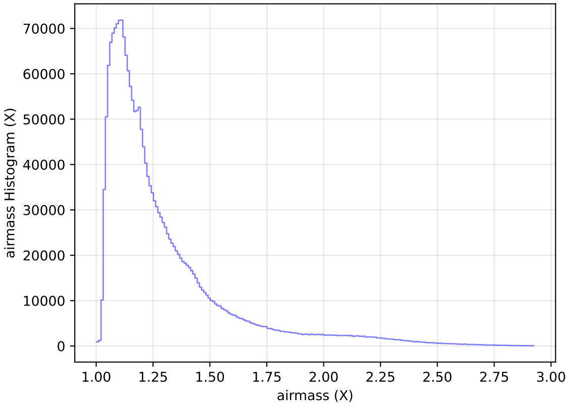
too_elab_r8_d2_griz_v3.4_10yrs WFD all bands: airmass Histogram
