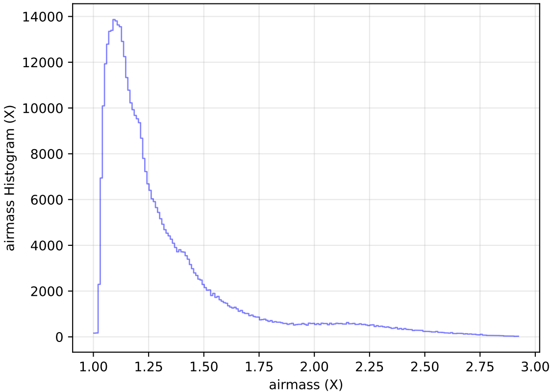
too_elab_r8_d2_griz_v3.4_10yrs All sky z band: airmass Histogram
