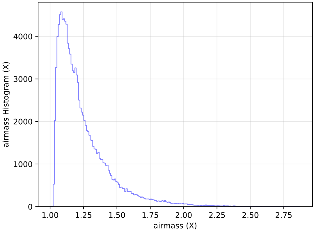
too_elab_r8_d2_griz_v3.4_10yrs All sky u band: airmass Histogram
