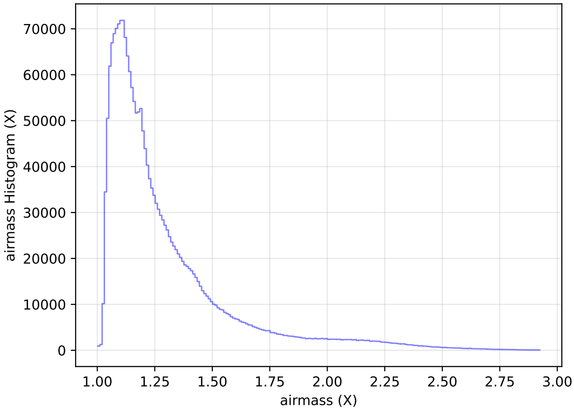
too_elab_r8_d2_griz_v3.4_10yrs All sky all bands: airmass Histogram
