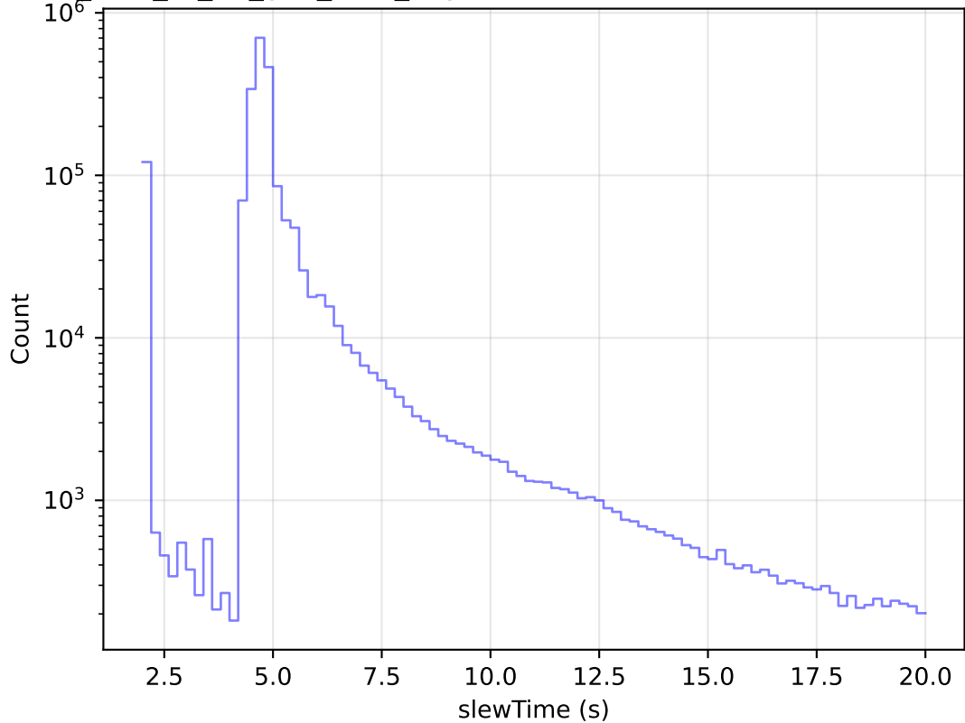
too_elab_r8_d2_griz_v3.4_10yrs All visits: Zoom Slew Time Histogram
