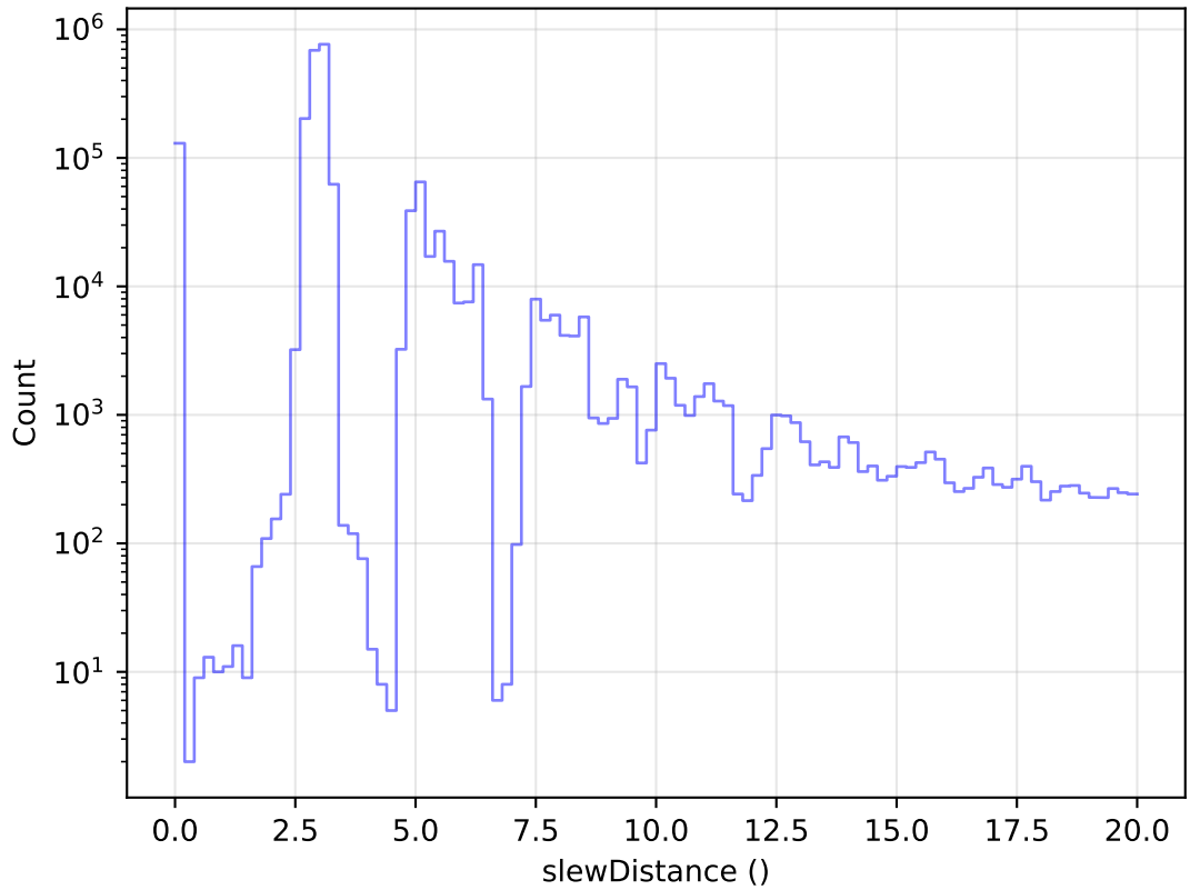
too_elab_r8_d2_griz_v3.4_10yrs All visits: Zoom Slew Distance Histogram
