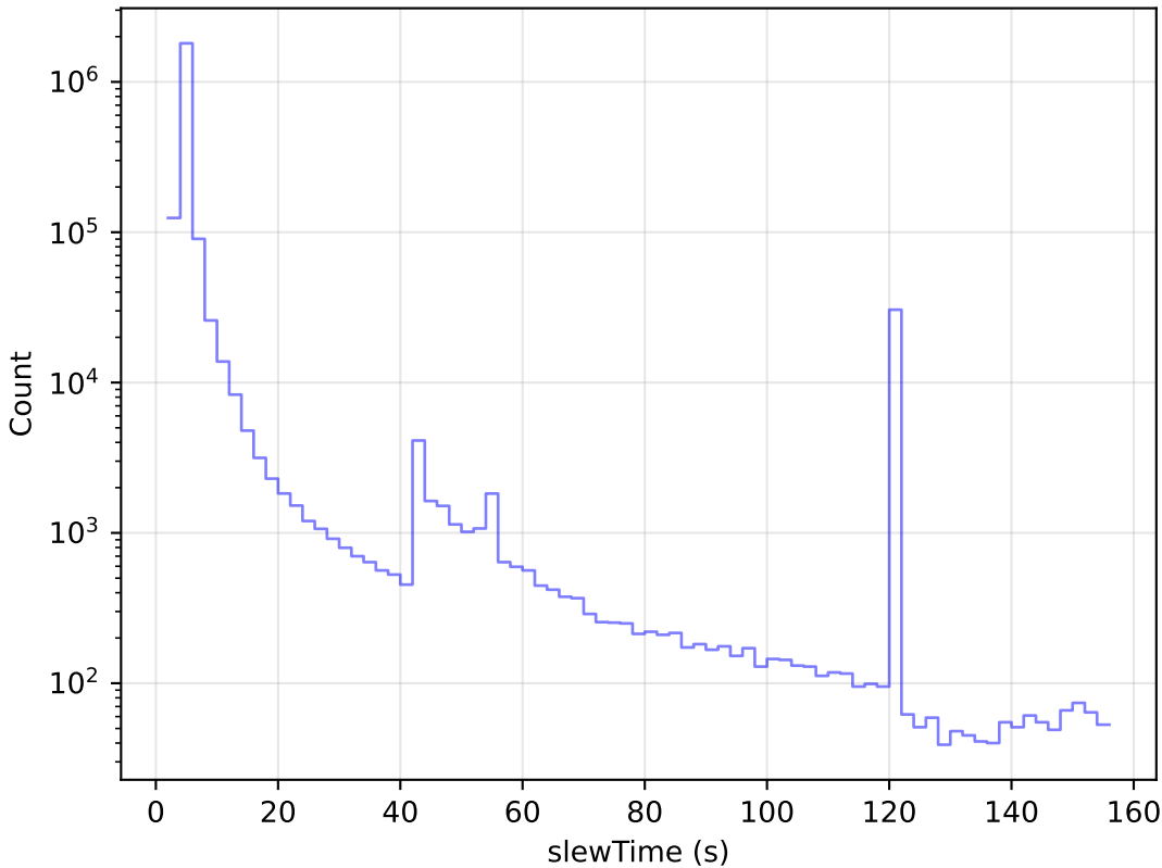
too_elab_r8_d2_griz_v3.4_10yrs All visits: Slew Time Histogram
