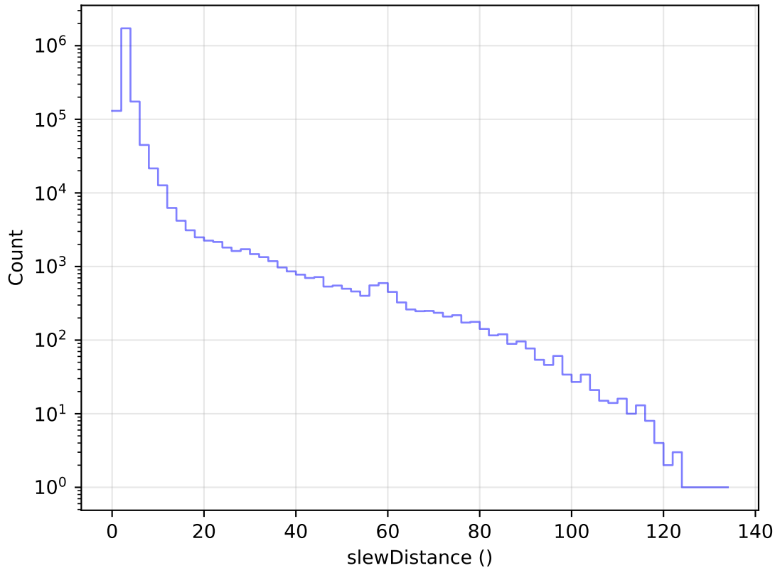
too_elab_r8_d2_griz_v3.4_10yrs All visits: Slew Distance Histogram
