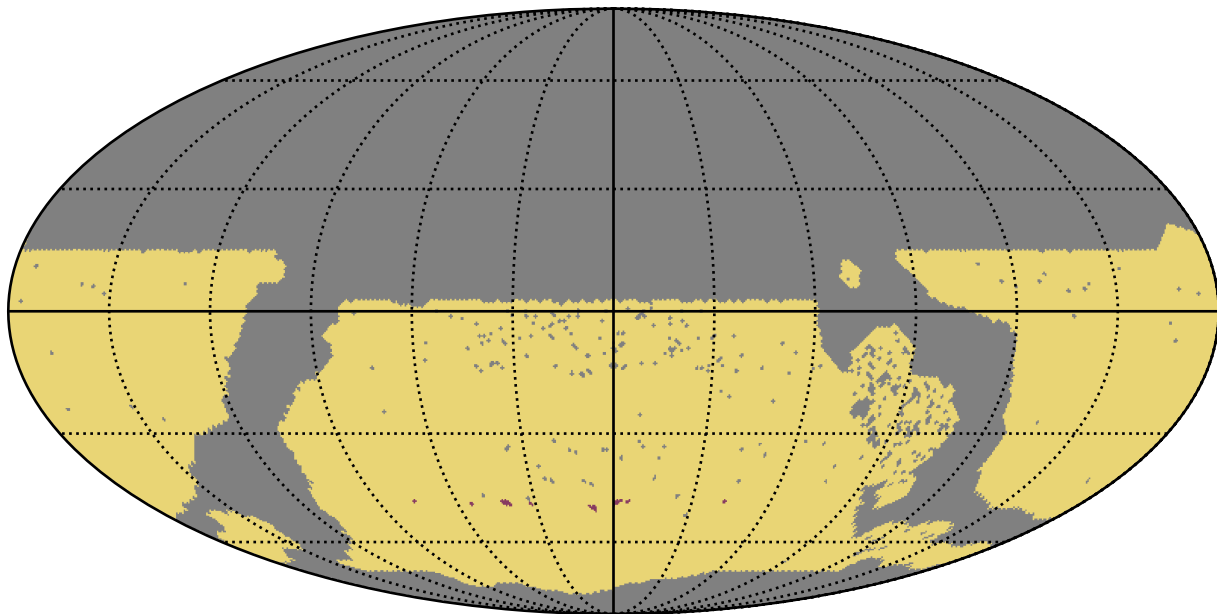
too_elab_r8_d2_griz_v3.4_10yrs WFD: RapidRevisits
