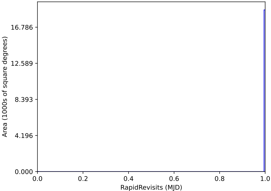
too_elab_r8_d2_griz_v3.4_10yrs WFD: RapidRevisits
