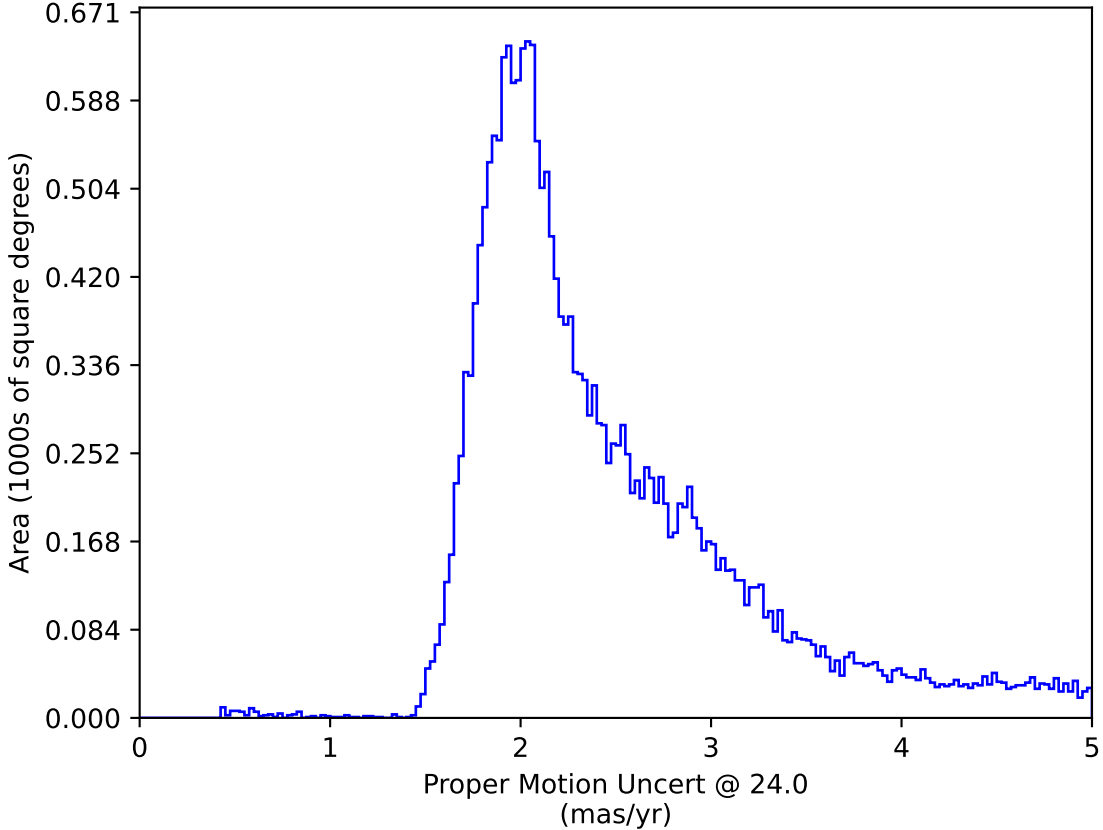
too_elab_r8_d2_griz_v3.4_10yrs All sky: Proper Motion Uncert @ 24.0
