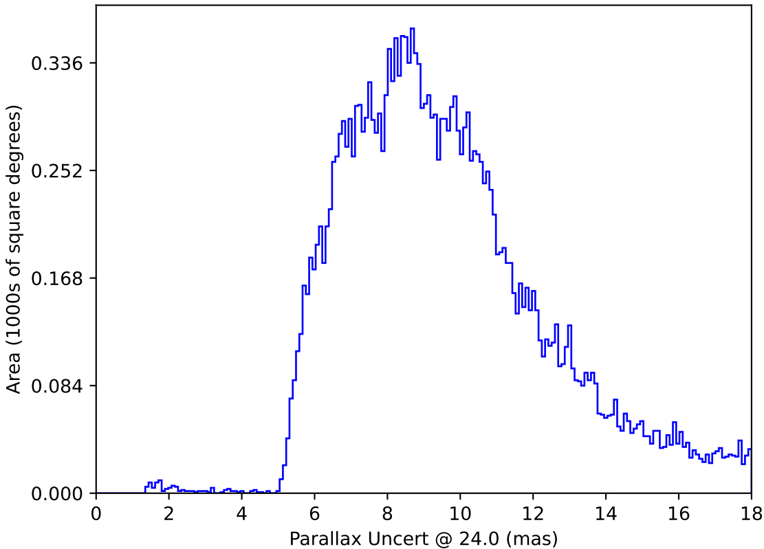
too_elab_r8_d2_griz_v3.4_10yrs All sky: Parallax Uncert @ 24.0
