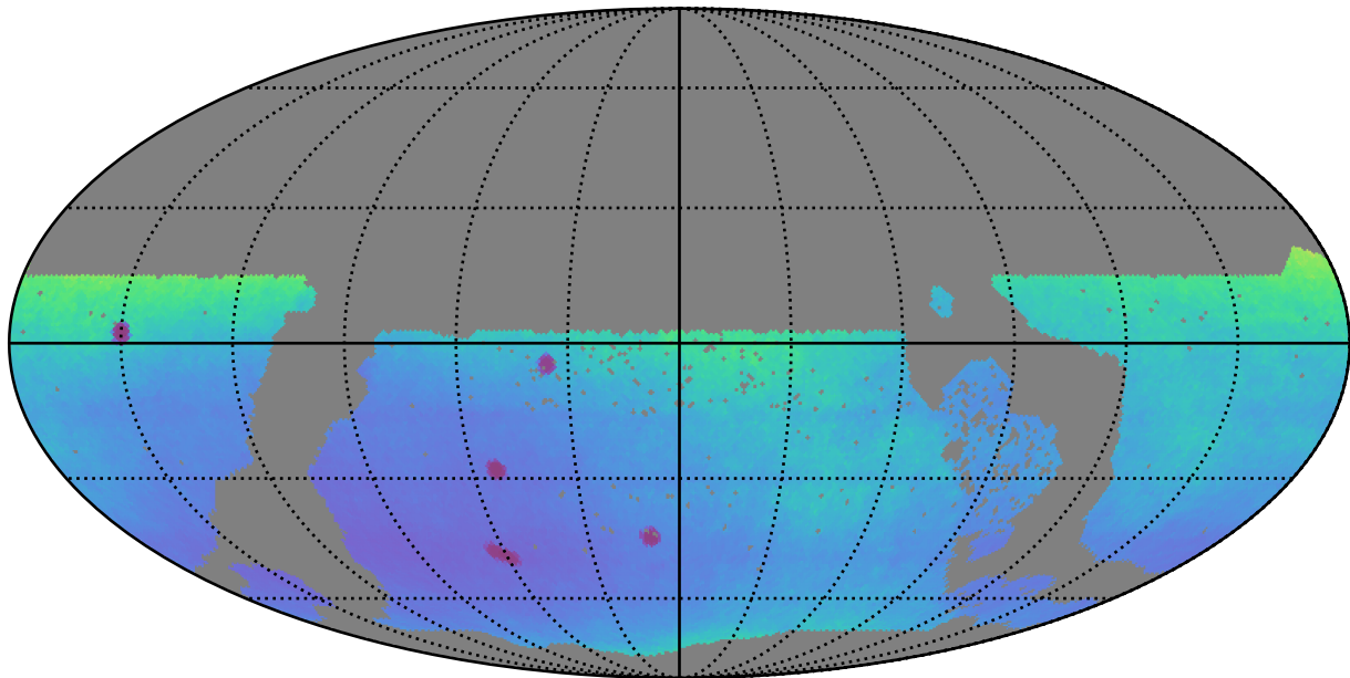
too_elab_r8_d2_griz_v3.4_10yrs WFD: Parallax Uncert @ 22.4
