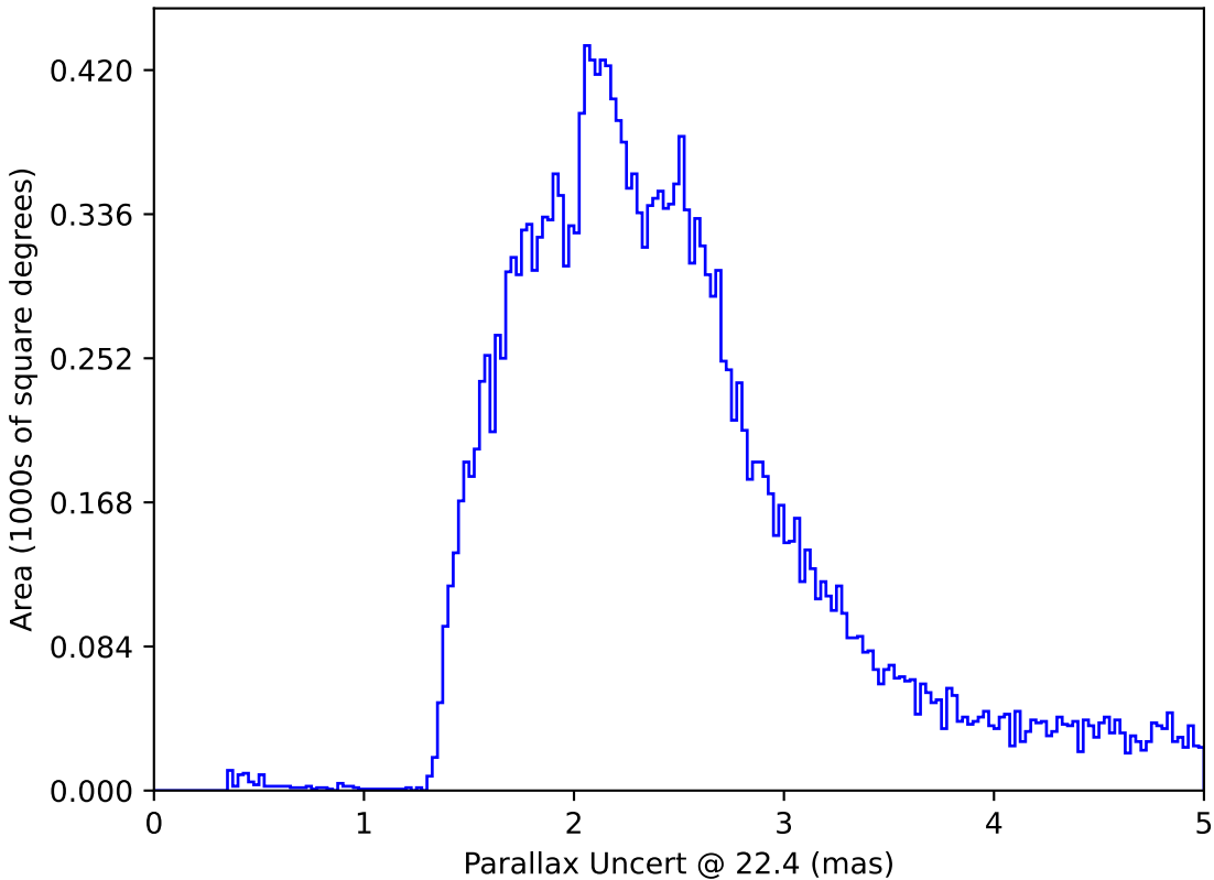
too_elab_r8_d2_griz_v3.4_10yrs All sky: Parallax Uncert @ 22.4
