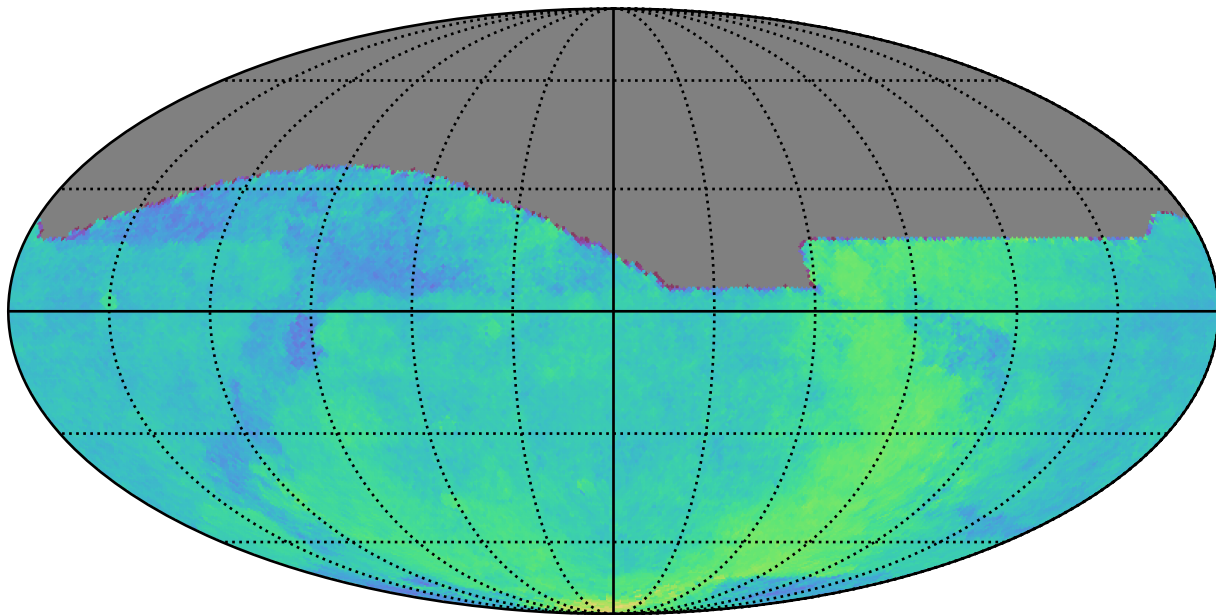
too_elab_r8_d2_griz_v3.4_10yrs All sky: Parallax Coverage @ 24.0
