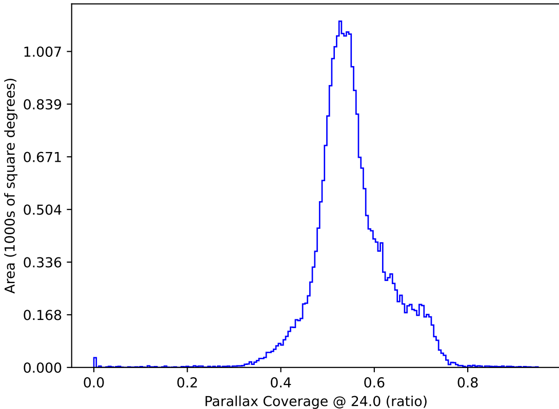
too_elab_r8_d2_griz_v3.4_10yrs All sky: Parallax Coverage @ 24.0
