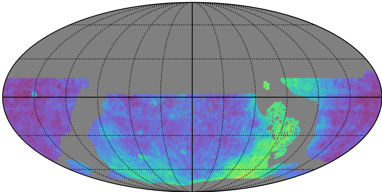
too_elab_r8_d2_griz_v3.4_10yrs WFD: Parallax Coverage @ 22.4
