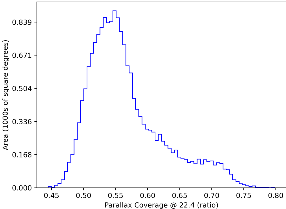
too_elab_r8_d2_griz_v3.4_10yrs WFD: Parallax Coverage @ 22.4
