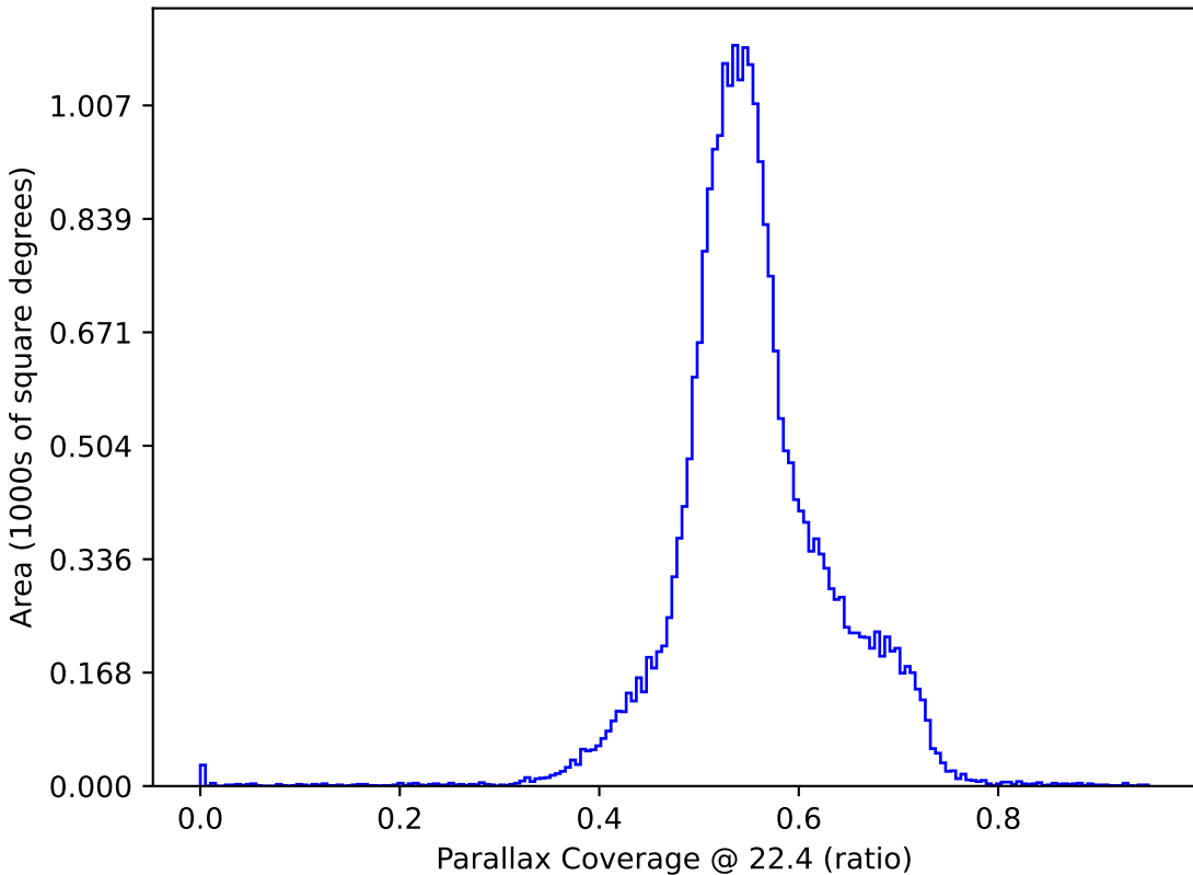
too_elab_r8_d2_griz_v3.4_10yrs All sky: Parallax Coverage @ 22.4
