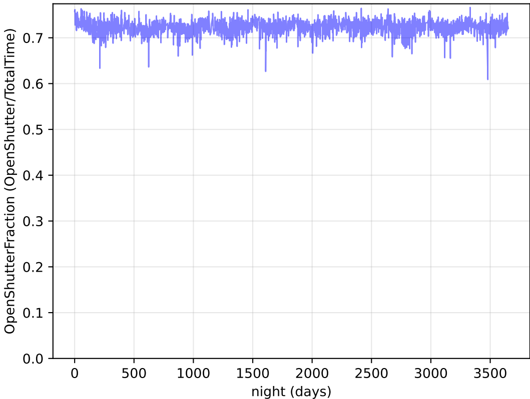
too_elab_r8_d2_griz_v3.4_10yrs Per night: OpenShutterFraction
