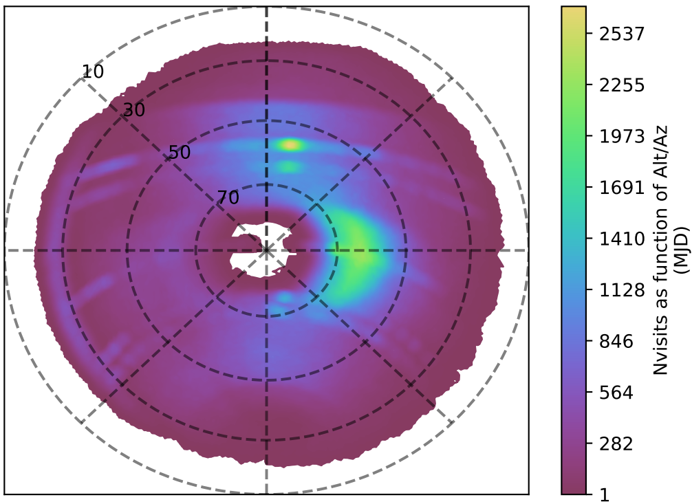
too_elab_r8_d2_griz_v3.4_10yrs r band: Nvisits as function of Alt/Az
