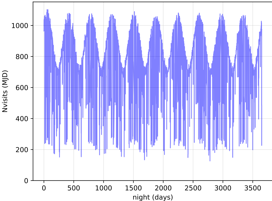
too_elab_r8_d2_griz_v3.4_10yrs All visits: Nvisits
