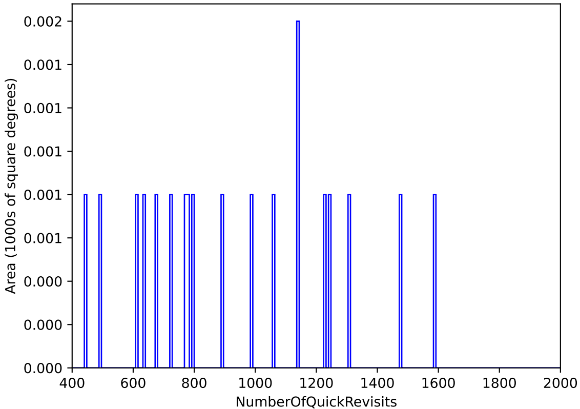
too_elab_r8_d2_griz_v3.4_10yrs WFD: NumberOfQuickRevisits
