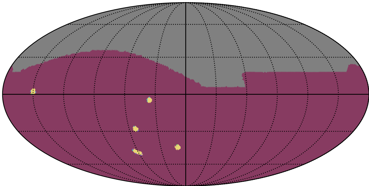
too_elab_r8_d2_griz_v3.4_10yrs All sky: NumberOfQuickRevisits
