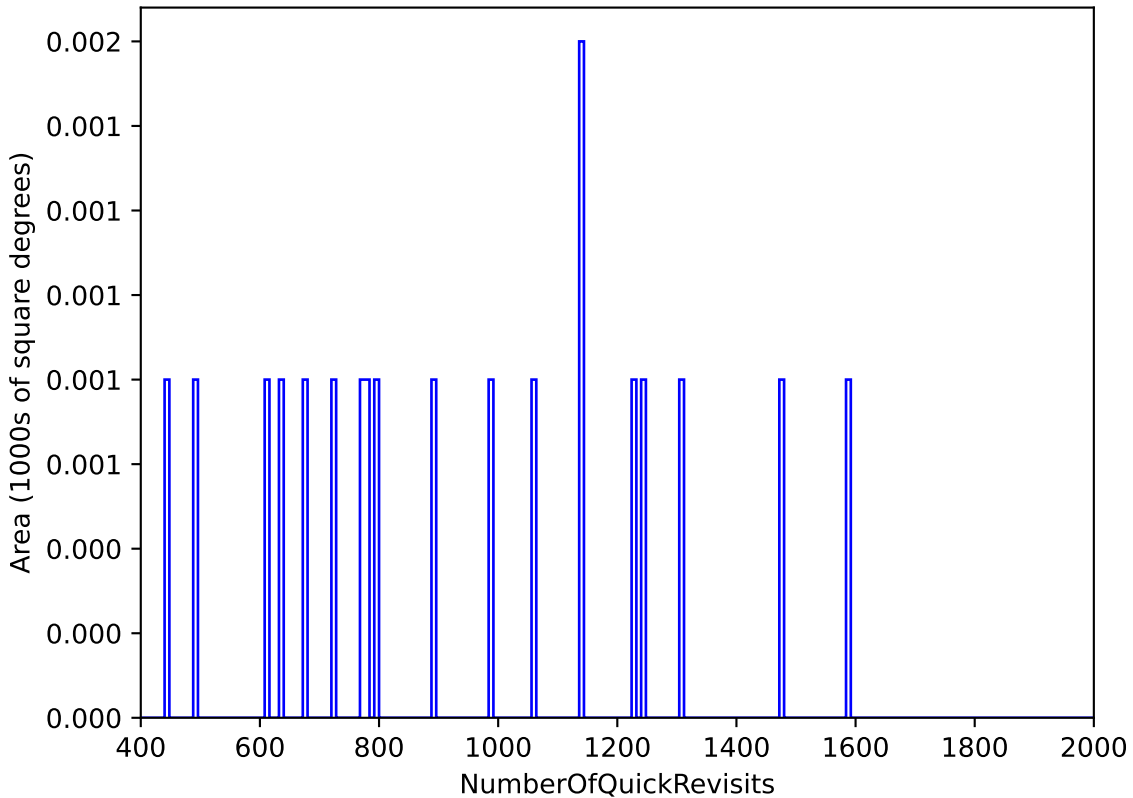
too_elab_r8_d2_griz_v3.4_10yrs All sky: NumberOfQuickRevisits
