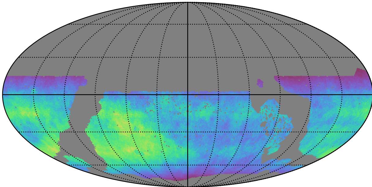
too_elab_r8_d2_griz_v3.4_10yrs WFD z band: Normalized Teff
