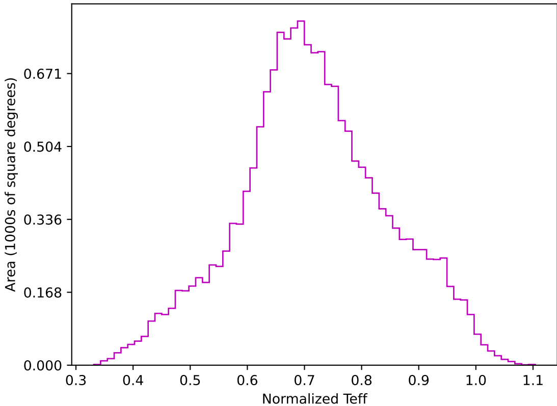
too_elab_r8_d2_griz_v3.4_10yrs WFD z band: Normalized Teff
