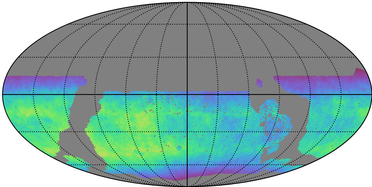
too_elab_r8_d2_griz_v3.4_10yrs WFD y band: Normalized Teff
