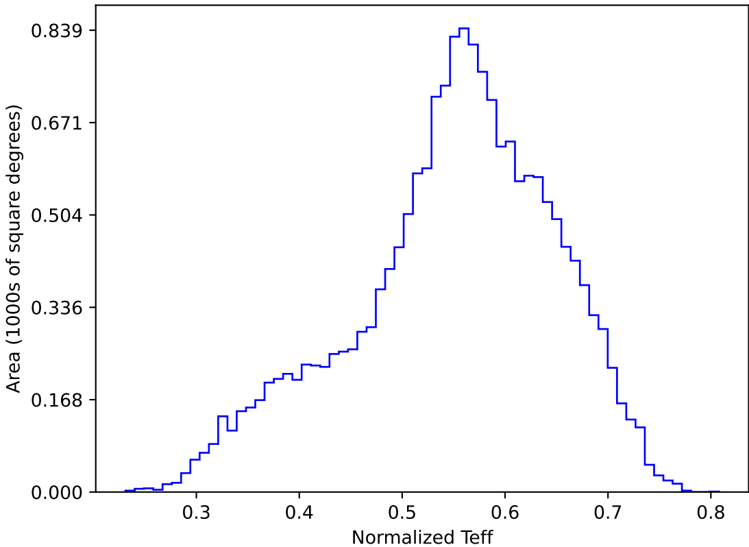
too_elab_r8_d2_griz_v3.4_10yrs WFD y band: Normalized Teff
