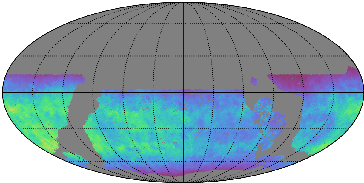
too_elab_r8_d2_griz_v3.4_10yrs WFD u band: Normalized Teff
