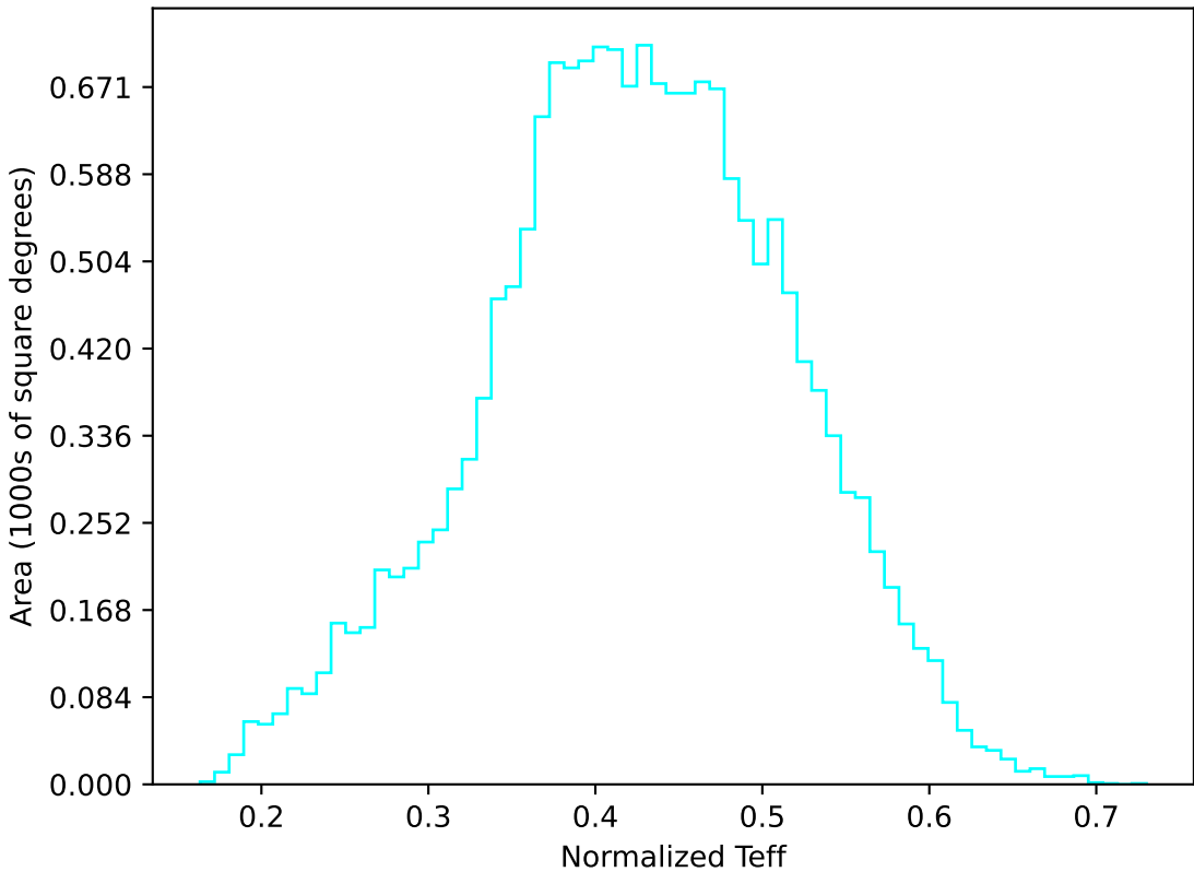
too_elab_r8_d2_griz_v3.4_10yrs WFD u band: Normalized Teff
