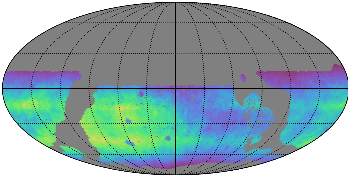
too_elab_r8_d2_griz_v3.4_10yrs WFD r band: Normalized Teff
