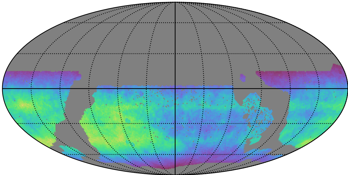
too_elab_r8_d2_griz_v3.4_10yrs WFD i band: Normalized Teff
