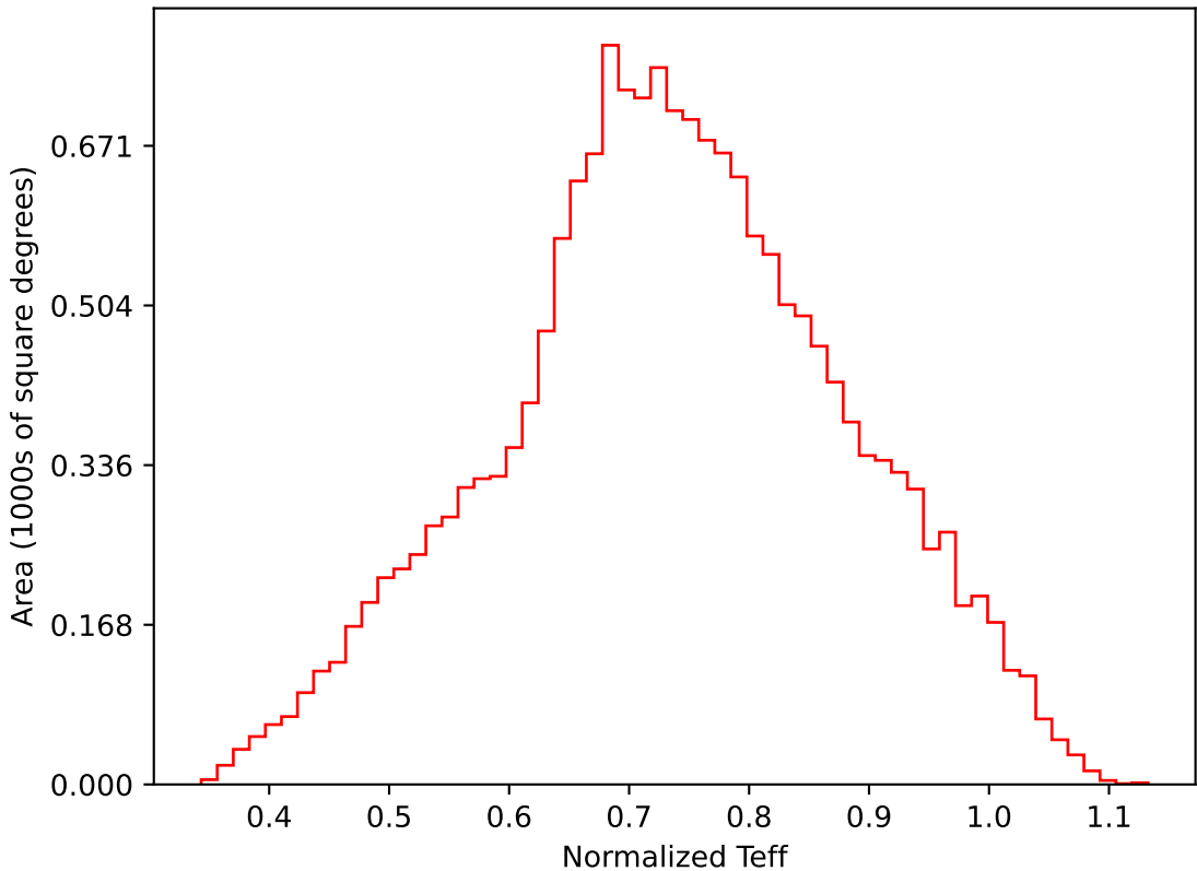
too_elab_r8_d2_griz_v3.4_10yrs WFD i band: Normalized Teff
