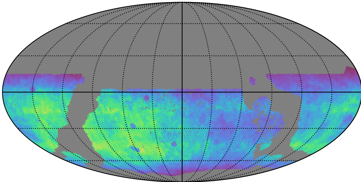
too_elab_r8_d2_griz_v3.4_10yrs WFD g band: Normalized Teff
