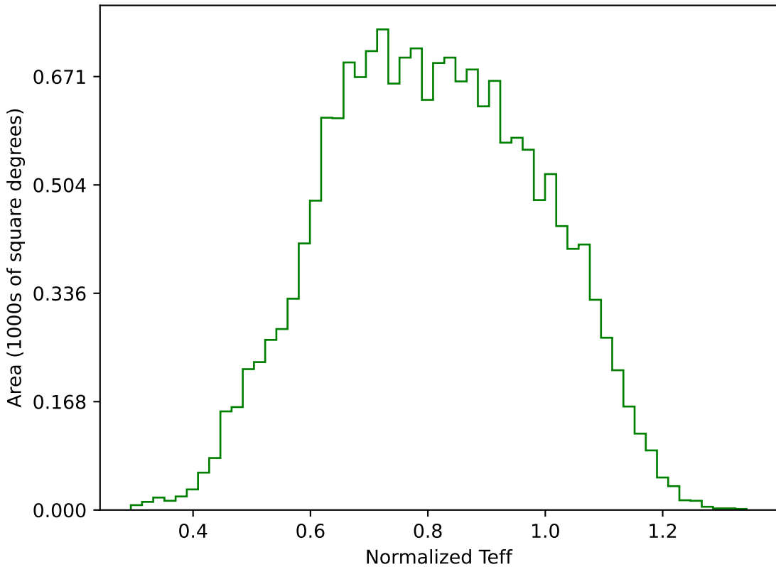
too_elab_r8_d2_griz_v3.4_10yrs WFD g band: Normalized Teff
