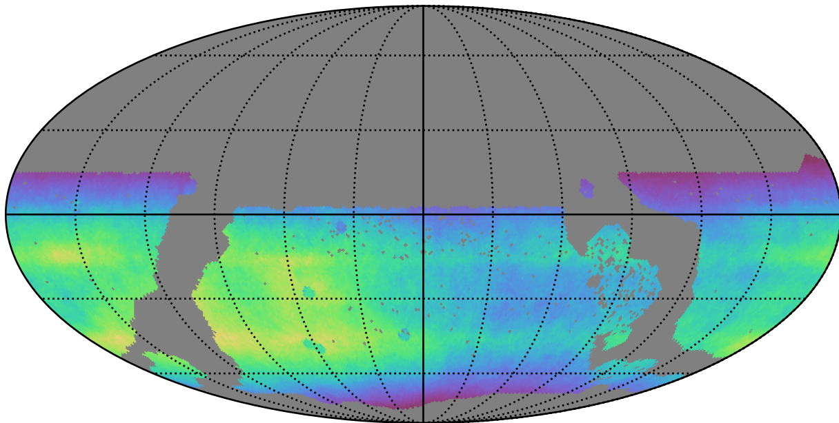
too_elab_r8_d2_griz_v3.4_10yrs WFD all bands: Normalized Teff
