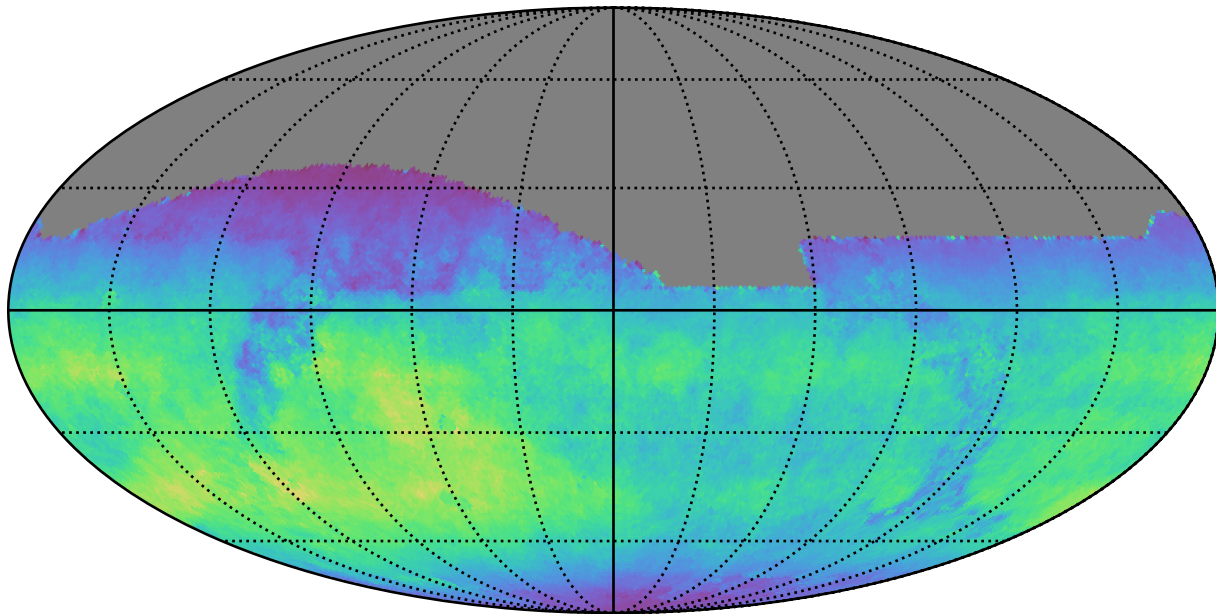
too_elab_r8_d2_griz_v3.4_10yrs All sky z band: Normalized Teff
