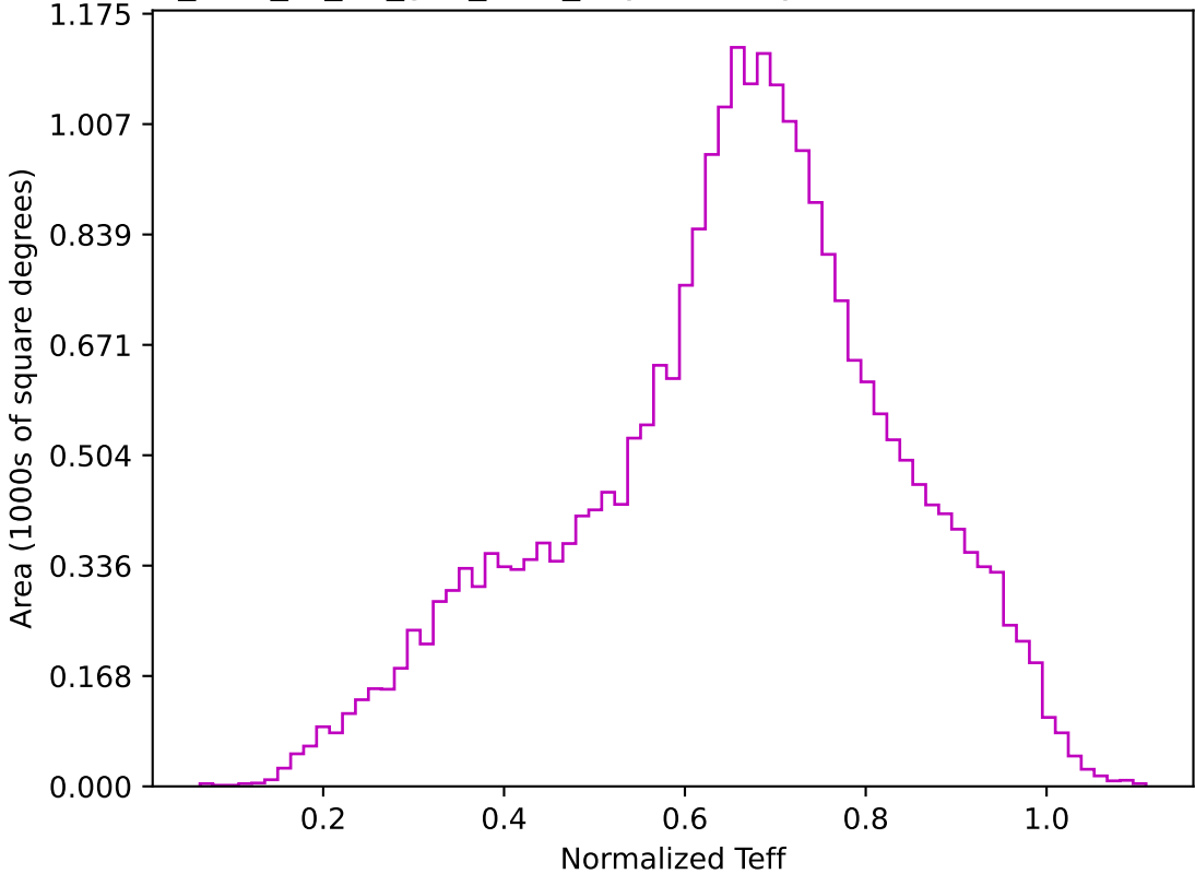
too_elab_r8_d2_griz_v3.4_10yrs All sky z band: Normalized Teff
