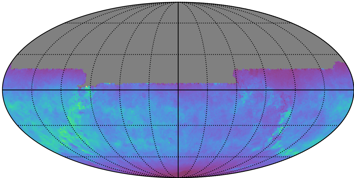
too_elab_r8_d2_griz_v3.4_10yrs All sky u band: Normalized Teff
