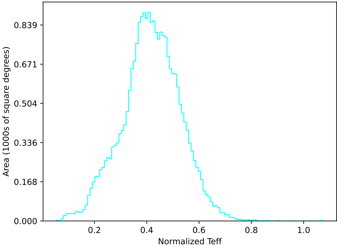
too_elab_r8_d2_griz_v3.4_10yrs All sky u band: Normalized Teff
