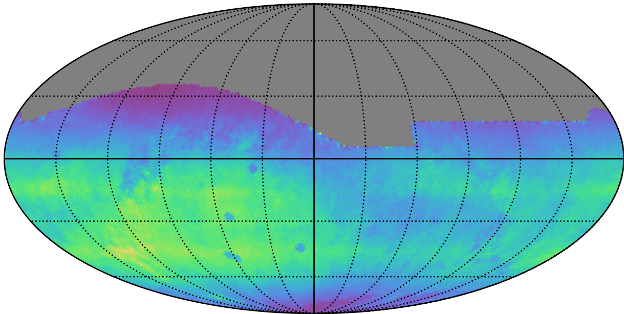
too_elab_r8_d2_griz_v3.4_10yrs All sky r band: Normalized Teff
