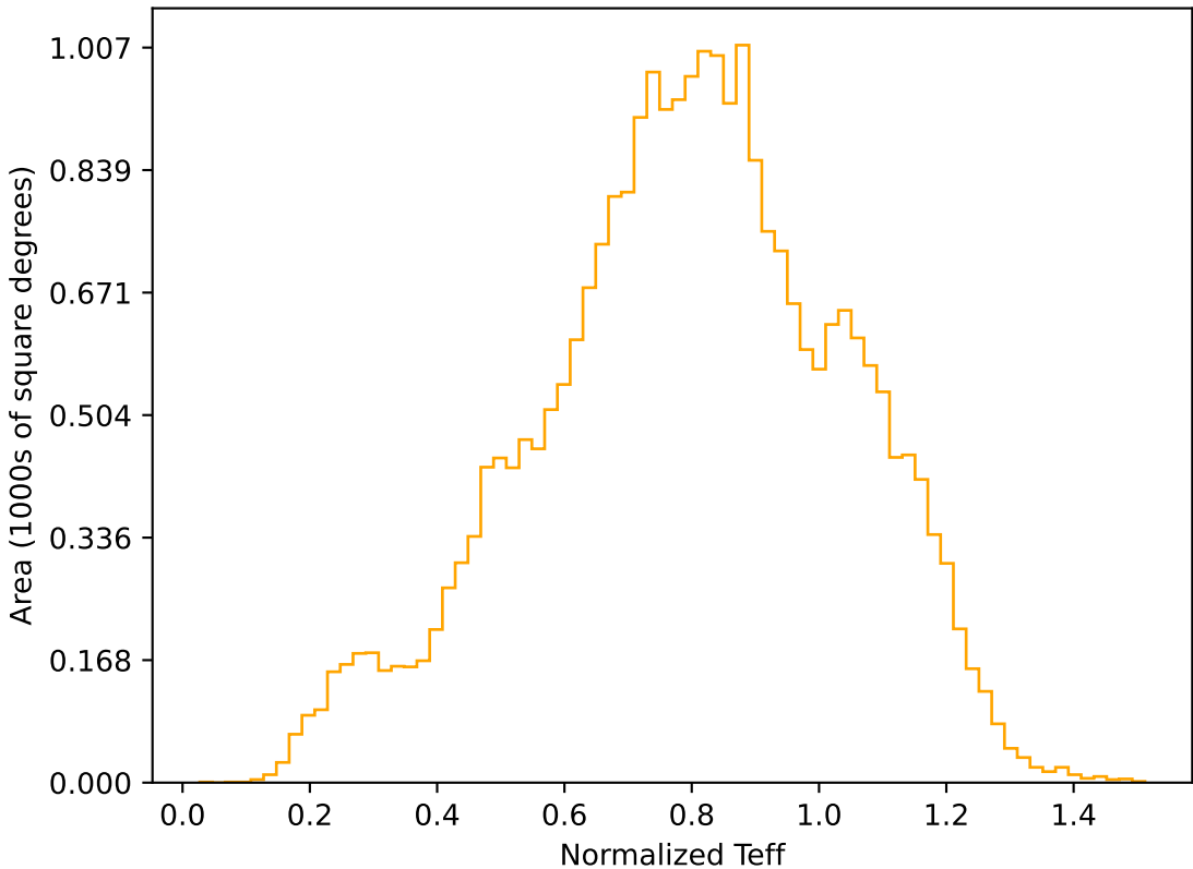
too_elab_r8_d2_griz_v3.4_10yrs All sky r band: Normalized Teff
